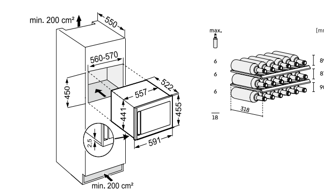
Installation Diagram
