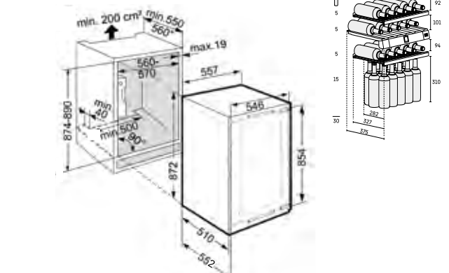
Installation Diagram
