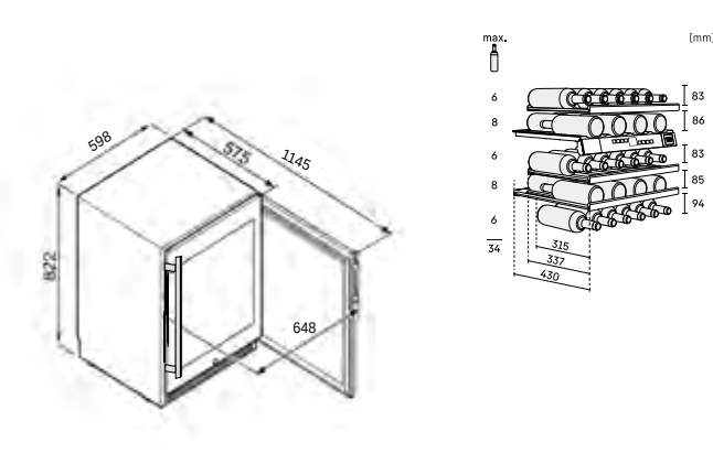
Installation Diagram
