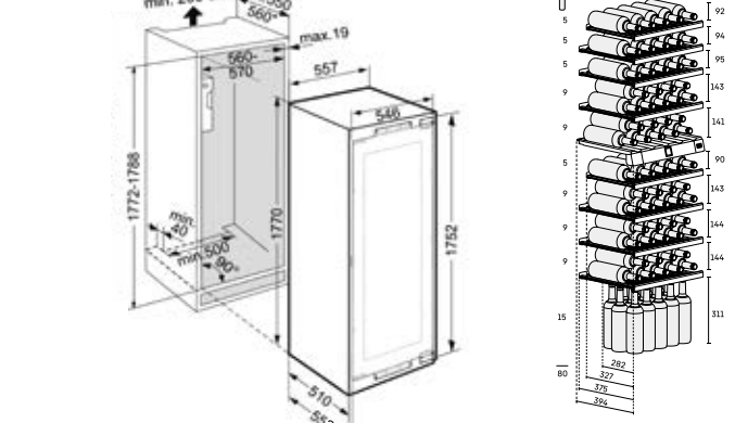
Installation Diagram
